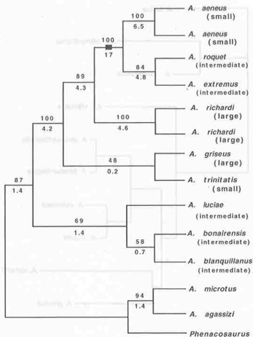
FIG. 4. The most parsimonious tree from the analysis of the combined dataset. Tree length = 1343.27. All notations are as in Figure 2.
