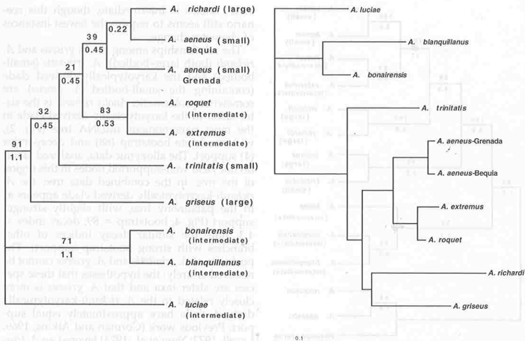
FIG. 3. (A) The most parsimonious tree resulting from analysis of the allozymic data. Specimens and data are taken from Yang et al. (1974). Tree length = 34.64. Bootstrap and decay index values shown as in Figure 2. Where no bootstrap value is shown, the branch did not appear in the bootstrap consensus tree. (B) The tree resulting from the neighbor-joining analysis of the allozymic data using Rogers (1972) genetic distances.
