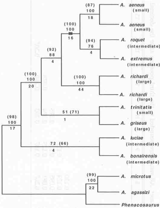
FIG. 2. The most parsimonious tree based on analysis of the mtDNA dataset. Tree length = 1307. Bootstrap values are shown above branches, decay index values below. Bootstrap values resulting from maximum-likelihood analysis are shown in parentheses. The black rectangle marks the origin of the derived karyotype 2n = 34 .
